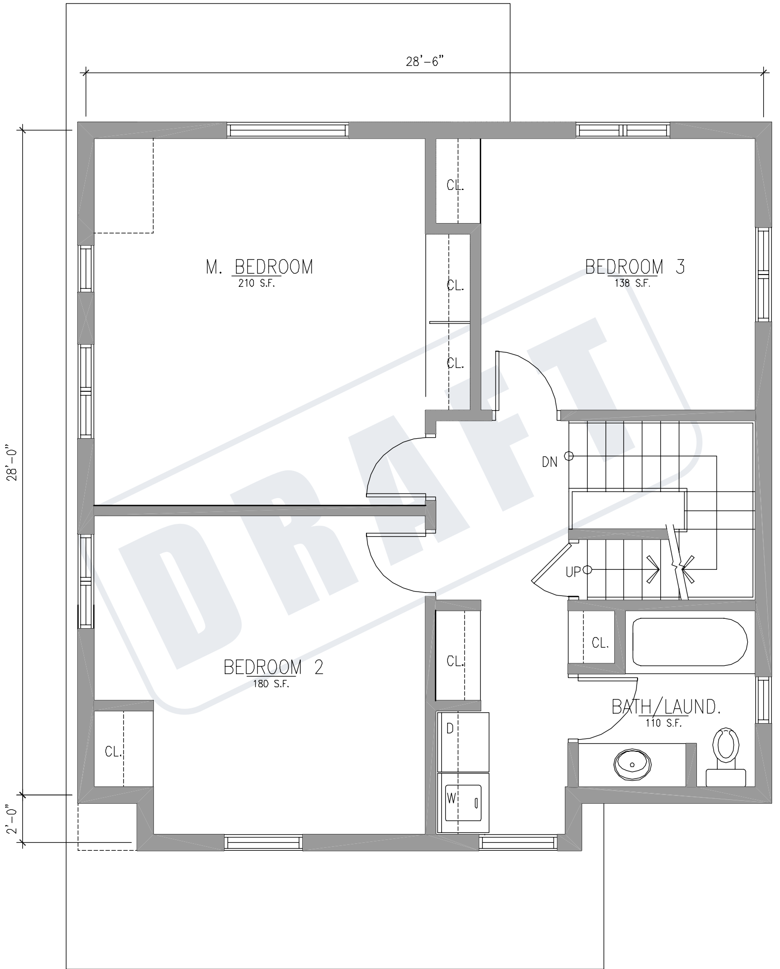
6 SECOND FLOOR PLAN 1/4" = 1'-0"
